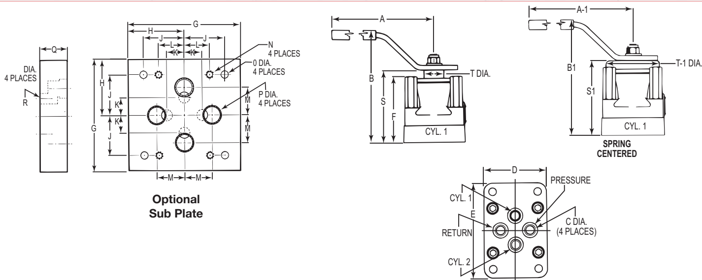
Valve Dimensions - inches (mm)
